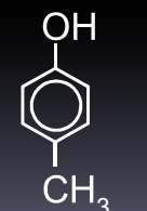
p -cresol
