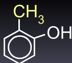
2-methylphenol
