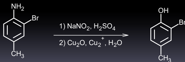
2-Bromo-4-methylphenol
