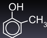
o -cresol
