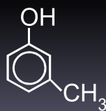
m -cresol
